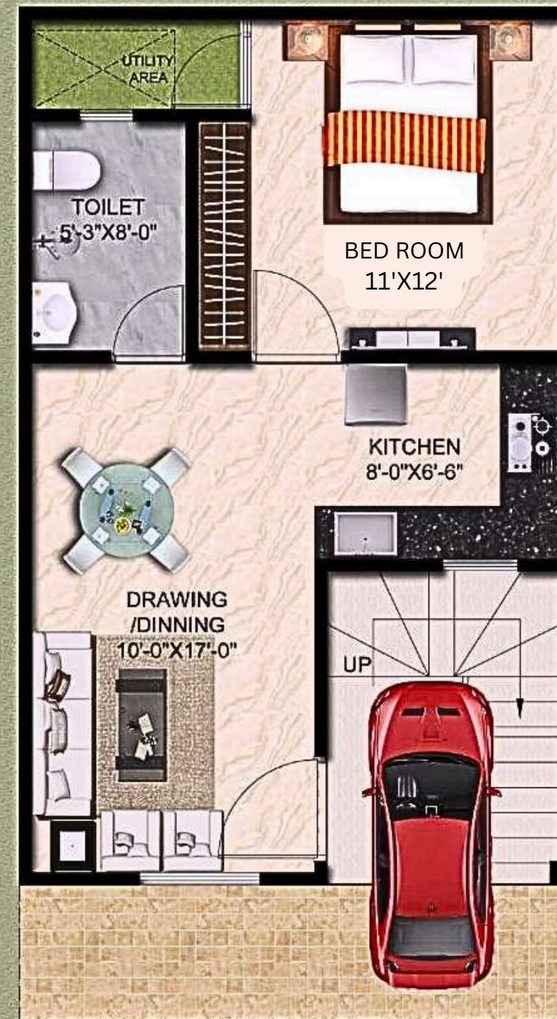
VILLA-GROUND FLOOR
